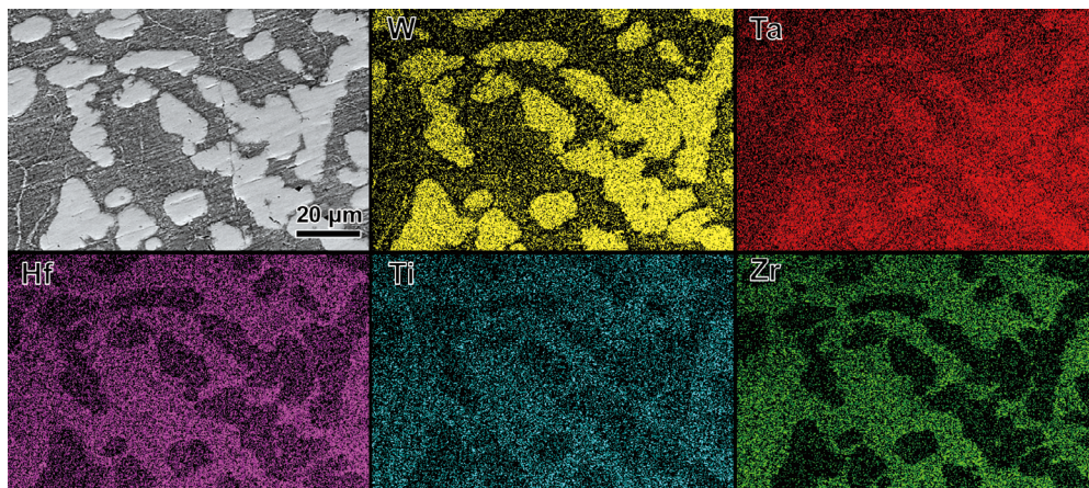
Fig. 3: SEM-EDS maps of as-cast WTaHfTiZr RHEA
