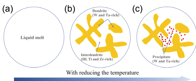
Fig. 6: Schematic diagram of microstructure formation during solidification of WTaHfTiZr RHEA
