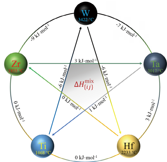
Fig. 5: Mixing enthalpy between any two elements and melting points for each element in WTaHfTiZr RHEA
