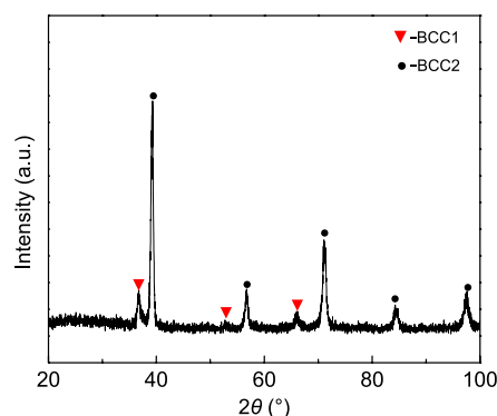
Fig. 1: XRD pattern of as-cast WTaHfTiZr RHEA
