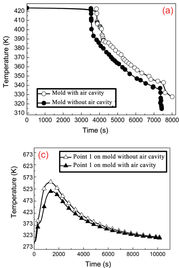
Fig. 7: Experimental results of insulation effect of air cavity on riser: (a) experimental temperature of Point B; (b) results of shrinkage; (c) cooling curves of Point 1
