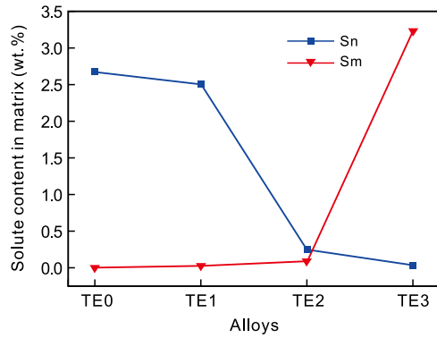
Fig. 5: Solubility variations of Sn and Sm in α-Mg matrix after solution treatment
