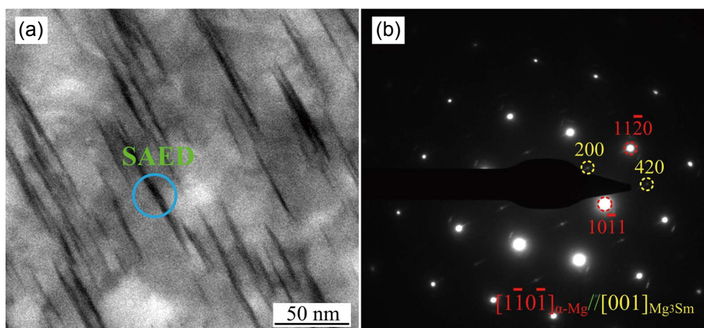
Fig. 8: TEM bright field image and corresponding SAED pattern of the peak-aged TE3 alloy: (a) bright field TEM image; (b) corresponding SAED patterns for the precipitates. The electron beam is parallel to the [1101]_{\alpha\text{-Mg}}
