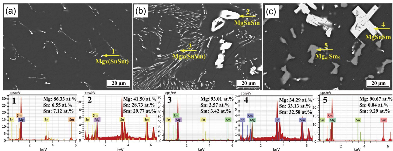
Fig. 4: SEM images of solution-treated alloys: (a) TE1, (b) TE2 and (c) TE3
