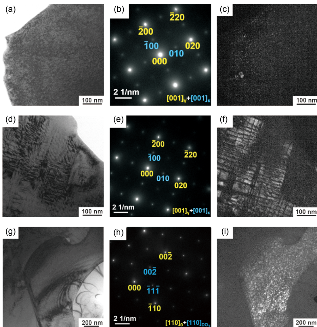
Fig. 8: TEM images of 0Cu steel strip after annealing at 700 °C for 3 h: (a) BF image of austenite; (b) SAED pattern along [001]_{\gamma} zone axis from (a); (c) DF image of \kappa -carbide particles; (d) BF image of austenite; (e) SAED pattern along [001]_{\gamma} zone axis from (d); (f) DF image of \kappa -carbide particles; (g) BF image of ferrite; (h) SAED pattern along [110]_{\delta} zone axis from (g); (i) DF image of \text{DO}_3 phase
